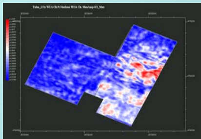
Maximum Amplitude in Interval of Interest
