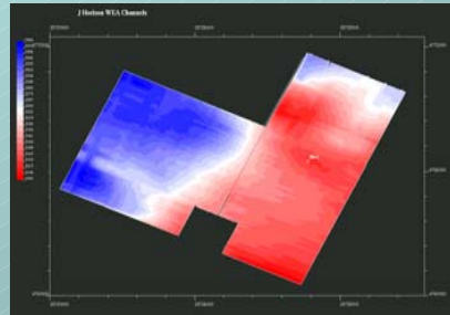
WEA Outline Overlay on Structure Map
