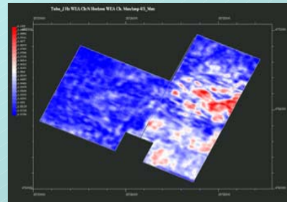
WEA Outline Overlay on Maximum Amplitude
