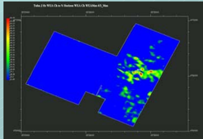
Maximum WEA in Interval of Interest
